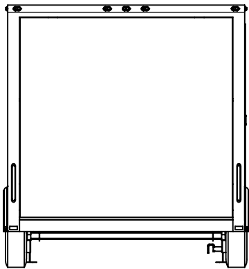
EXTERIOR REAR RAMP DOOR STANDARD SIZE 90"W x 84"H
