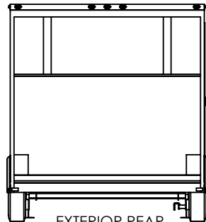
EXTERIOR REAR RAMP DOOR STANDARD SIZE 90"W x 78"H
