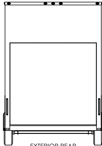
EXTERIOR REAR RAMP DOOR STANDARD SIZE 90" x 84"H
